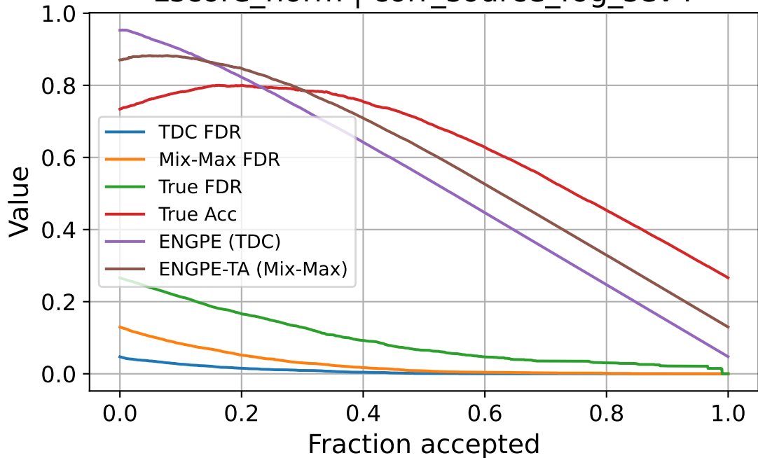
zscore_norm | corr_source_fog_sev4
