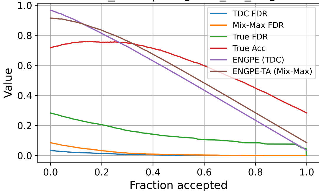
zscore_norm | imagenet_val_target
