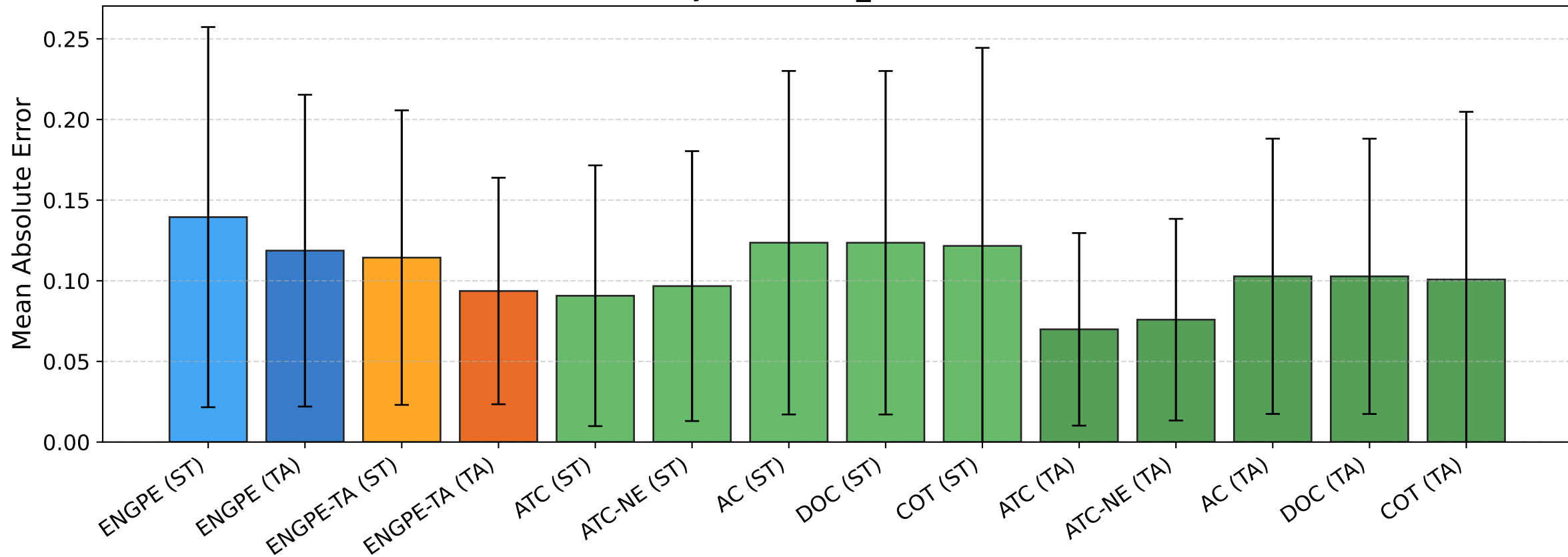
BREEDS entity30 [zscore_norm] — MAE [clean]
