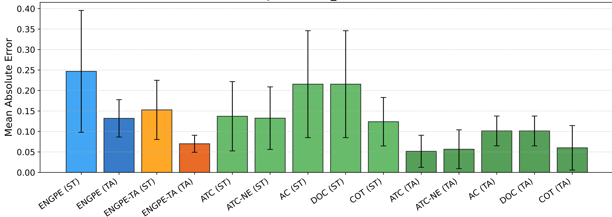
BREEDS entity30 [zscore_norm] — MAE [source]
