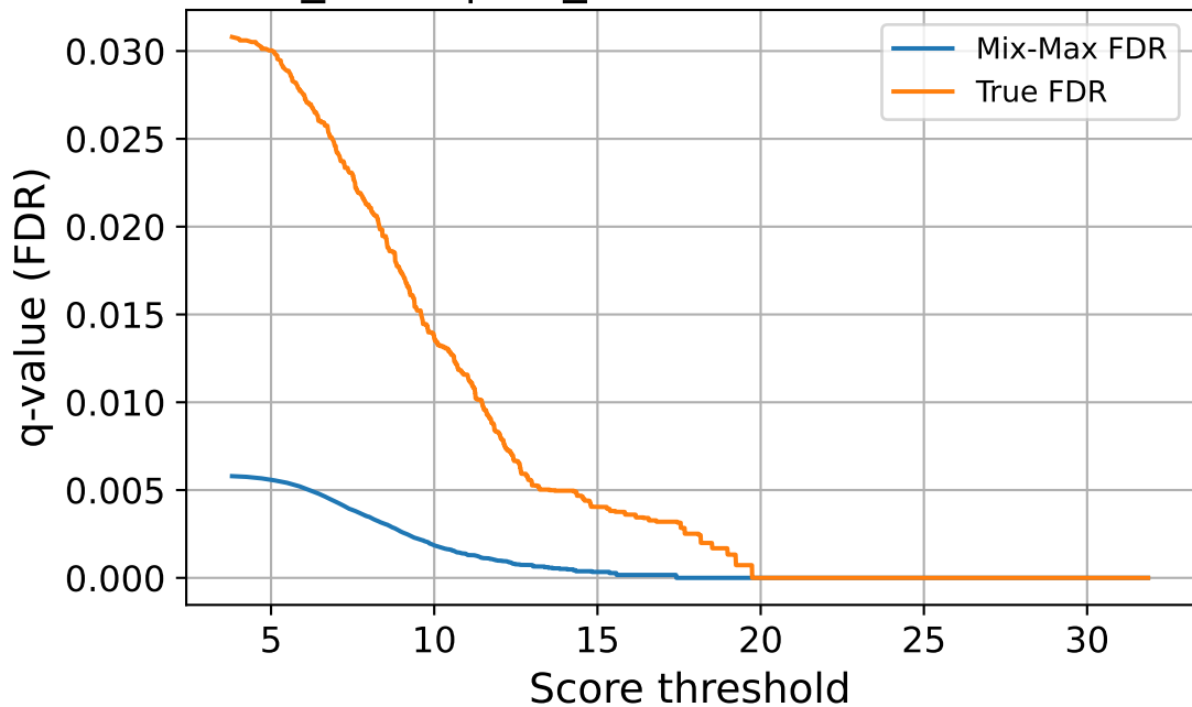
zscore_norm | val_source — FDR vs Threshold
