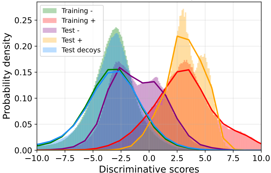
Score Distribution with Decoys for class 3
