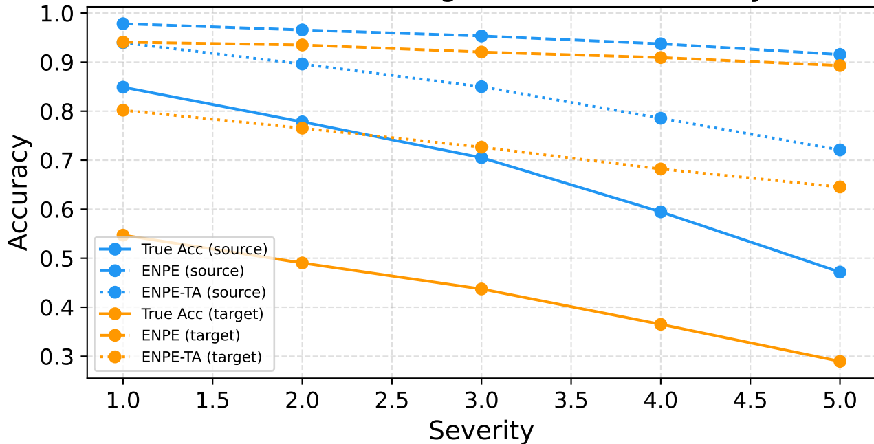
BREEDS nonliving26 — Acc vs Severity
