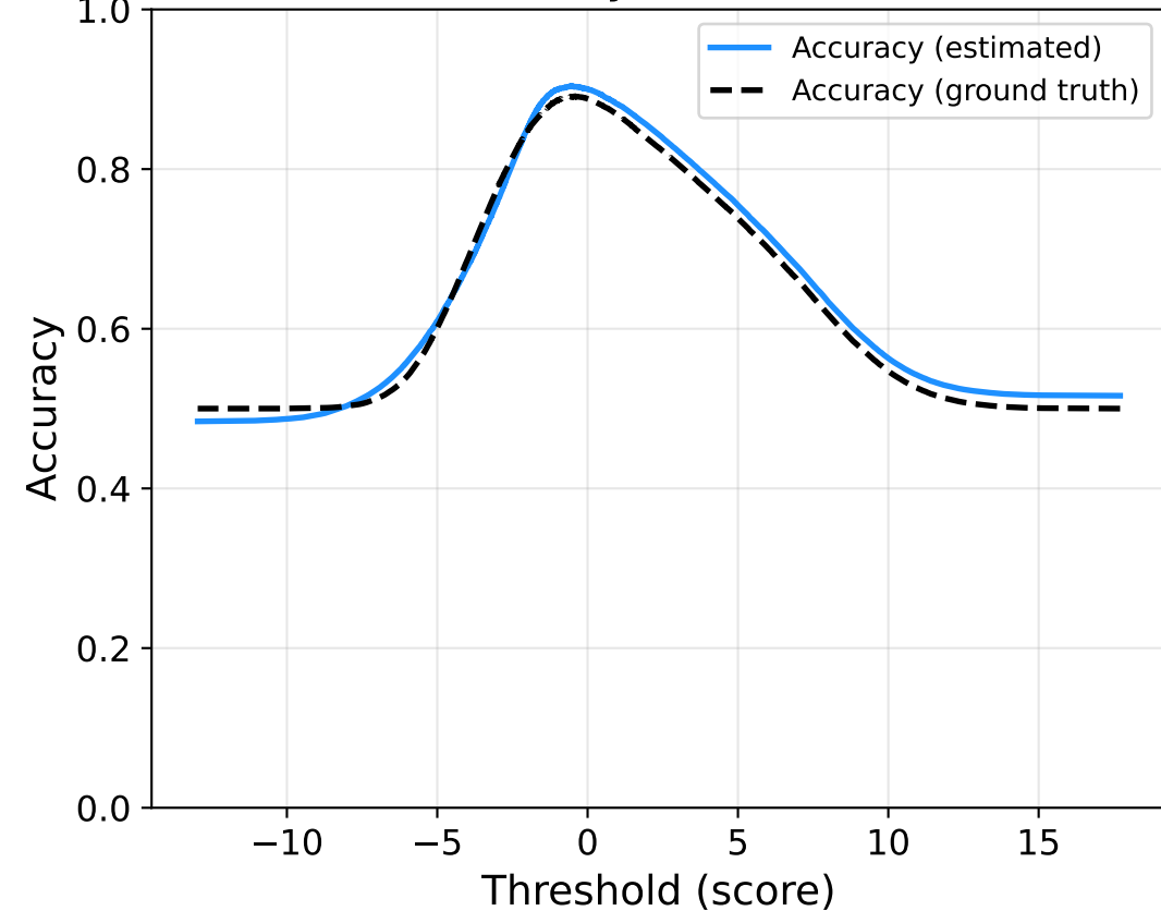
Accuracy Estimation
