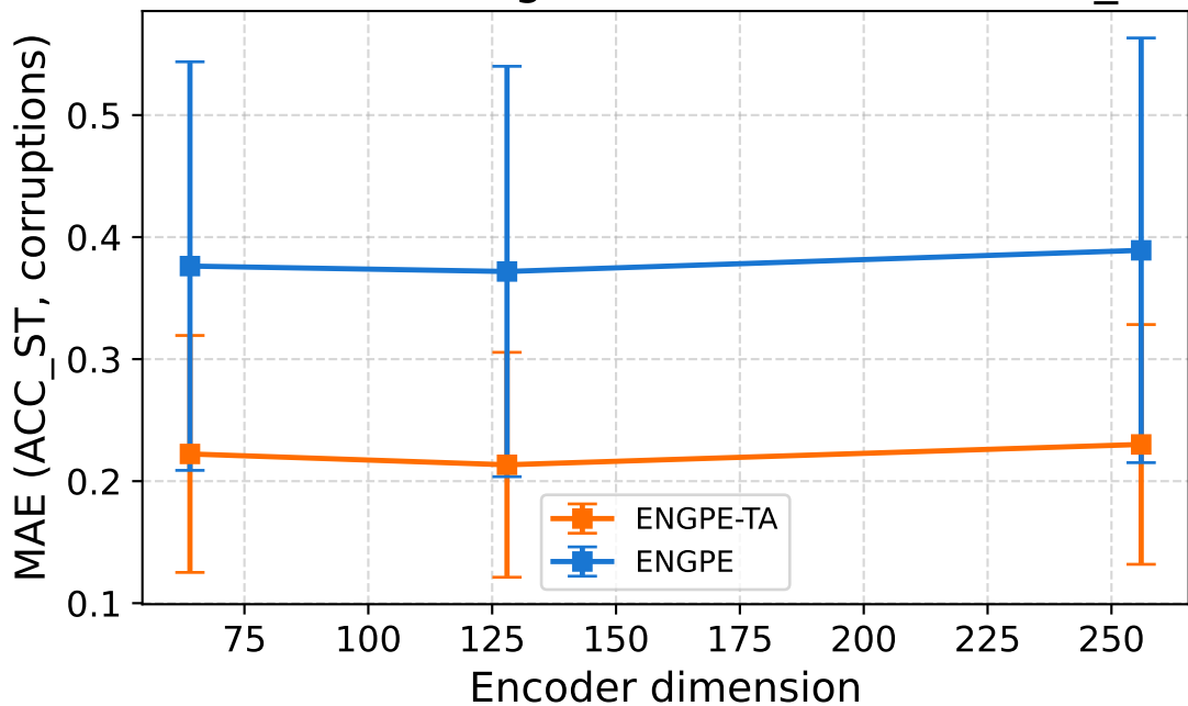
BREEDS nonliving26 — Ablation: encoder_dim
