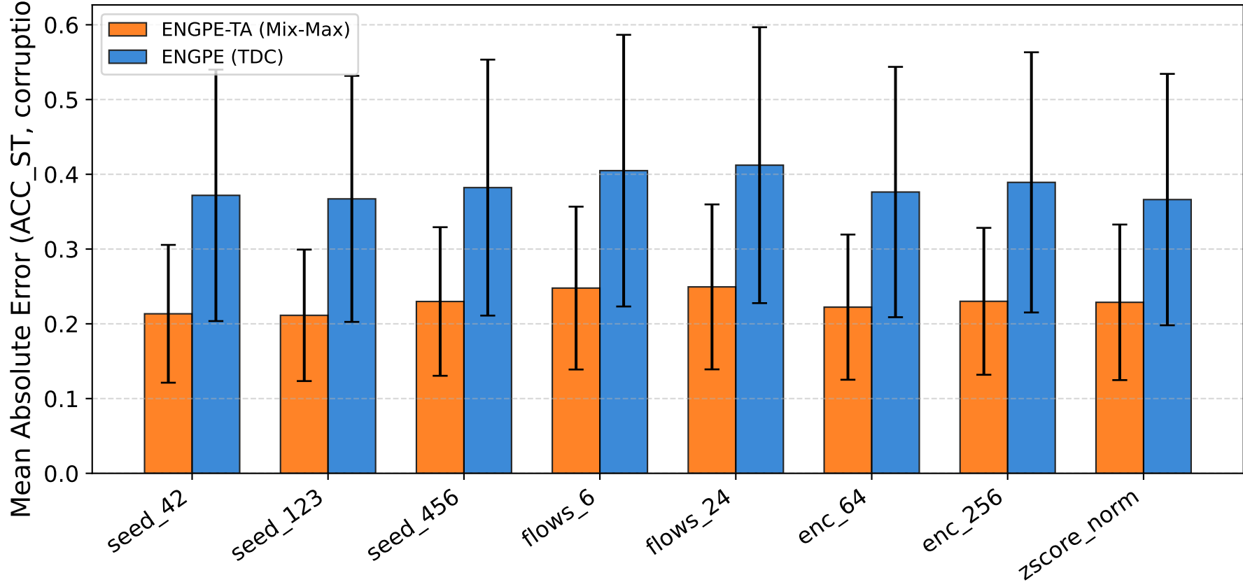
BREEDS nonliving26 — Ablation: MAE by Flow Config
