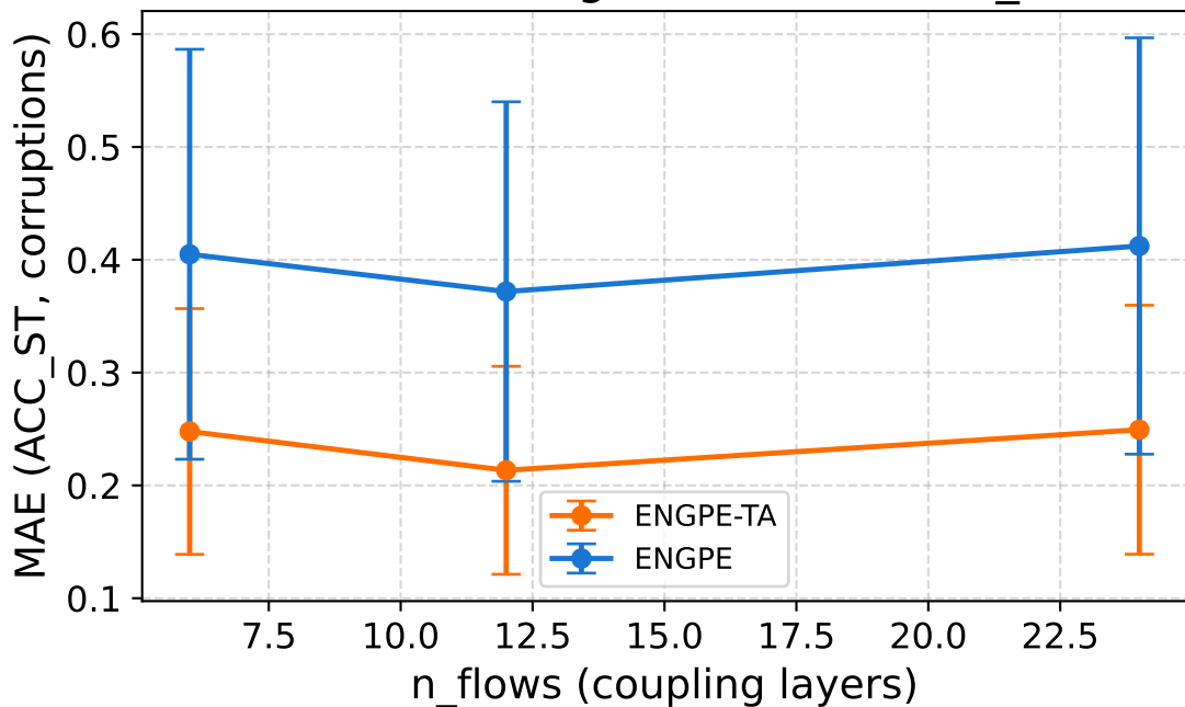
BREEDS nonliving26 — Ablation: n_flows
