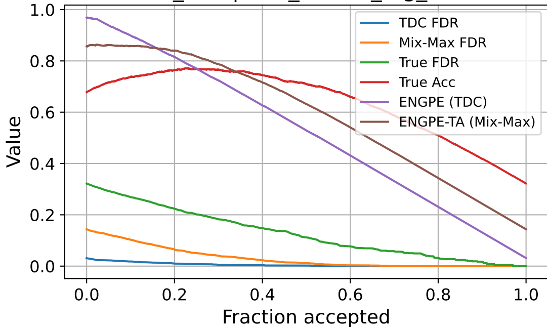
enc_256 | corr_source_fog_sev4
