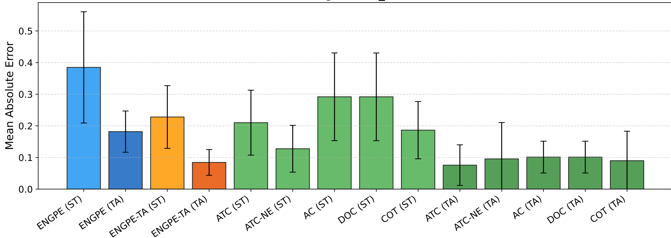
BREEDS nonliving26 [enc_256] — MAE [all]
