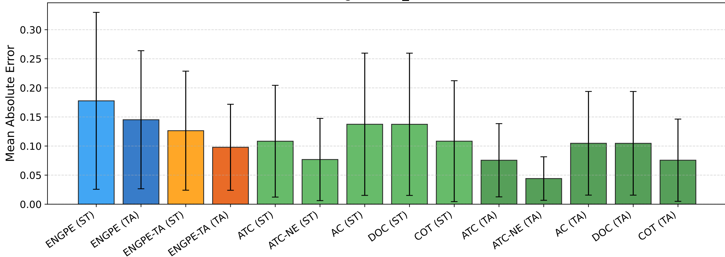
BREEDS nonliving26 [enc_256] — MAE [clean]
