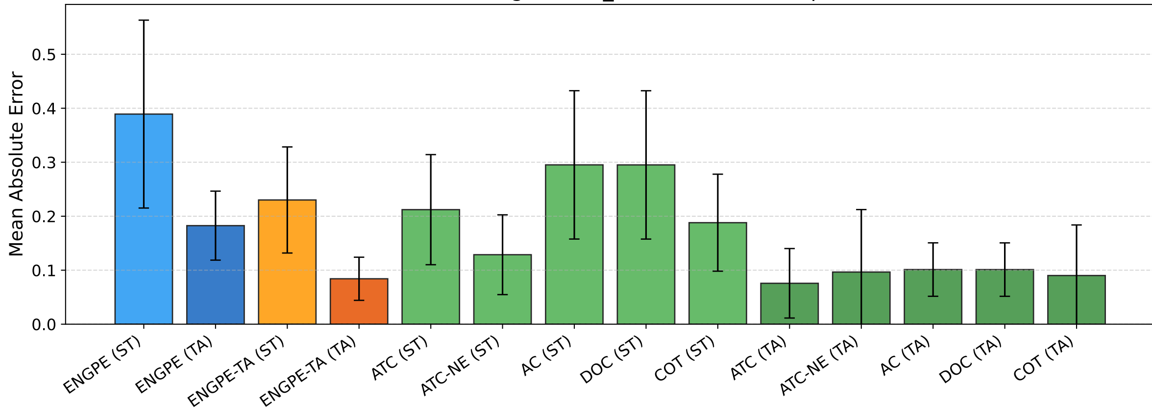
BREEDS nonliving26 [enc_256] — MAE [corruptions]
