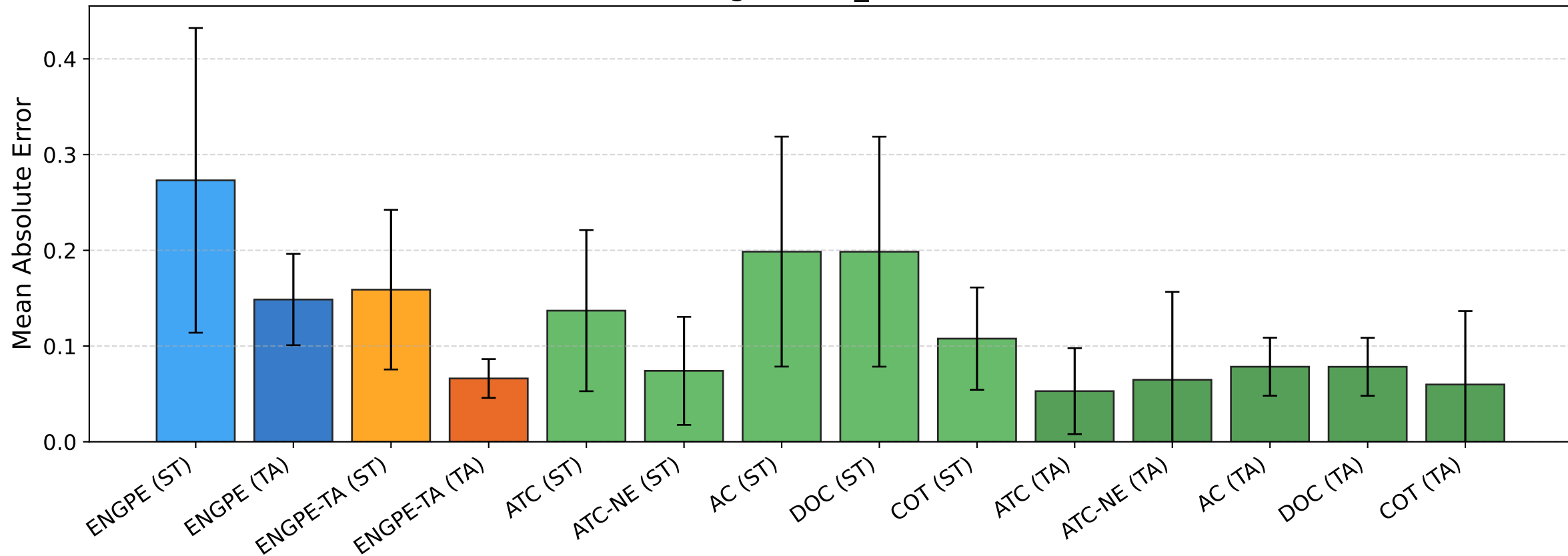
BREEDS nonliving26 [enc_256] — MAE [source]
