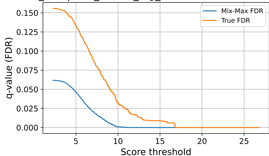
enc_256 | corr_source_fog_sev1 — FDR vs Threshold
