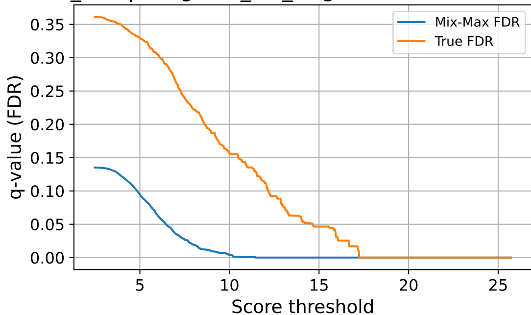
enc_256 | imagenet_val_target — FDR vs Threshold
