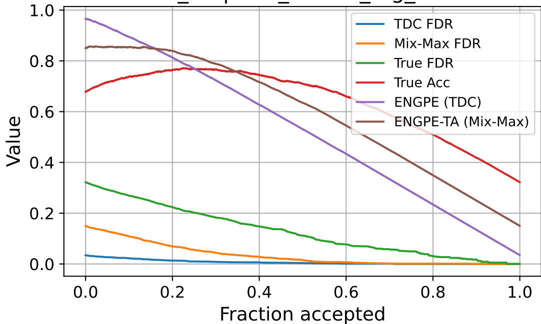
enc_64 | corr_source_fog_sev4
