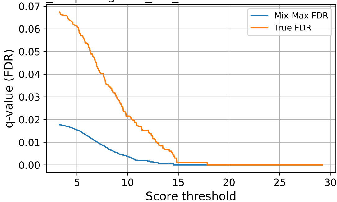
enc_64 | imagenet_val_source — FDR vs Threshold
