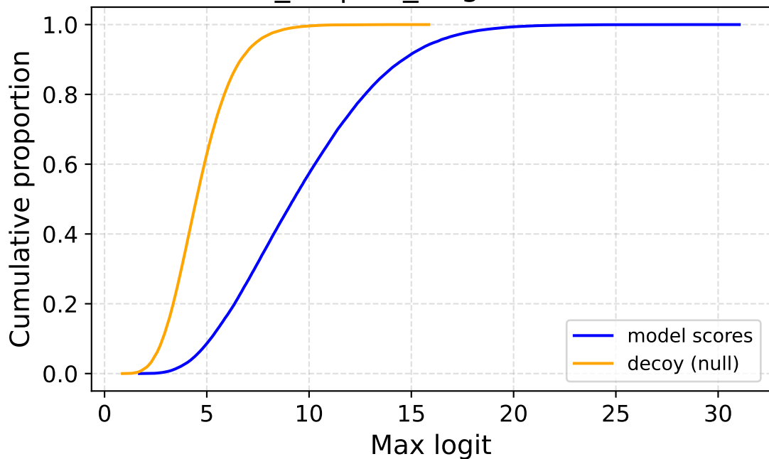
enc_64 | val_target — ECDF
