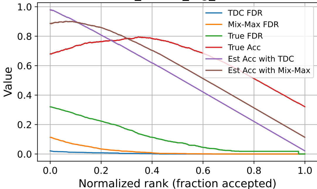
corr_source_fog_sev5
