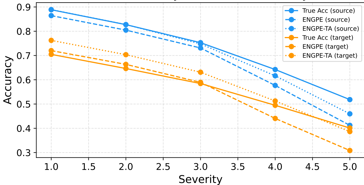
BREEDS entity13 — Acc vs Severity
