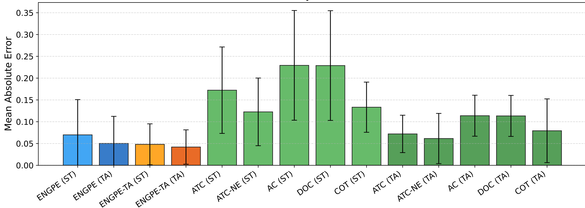
BREEDS entity13 — MAE [all]
