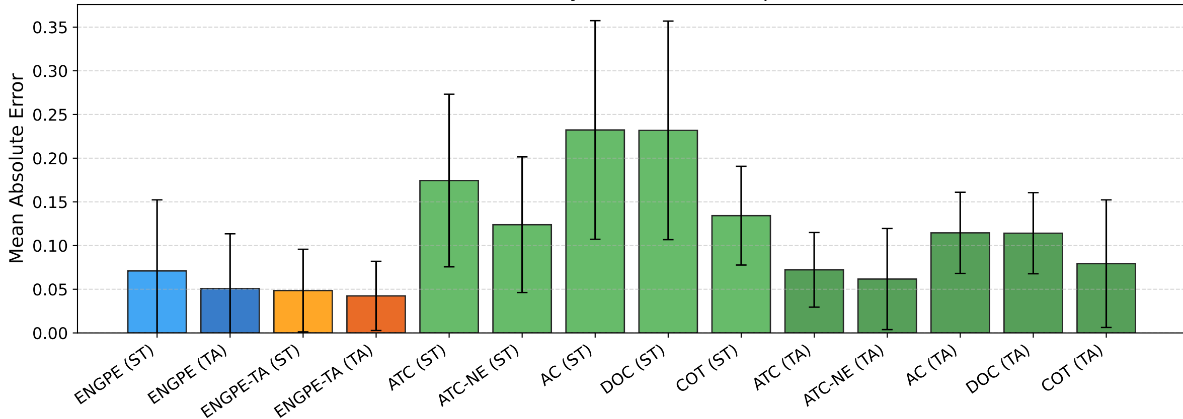
BREEDS entity13 — MAE [corruptions]
