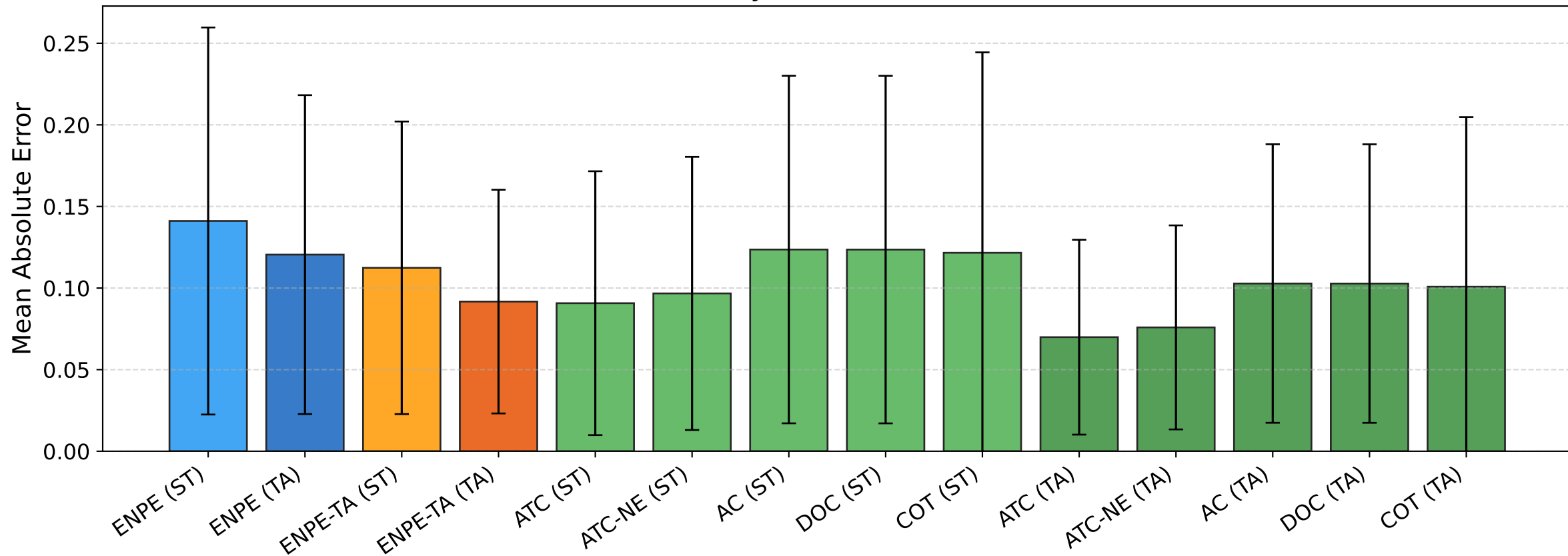
BREEDS entity30 — Mean Error [clean]
