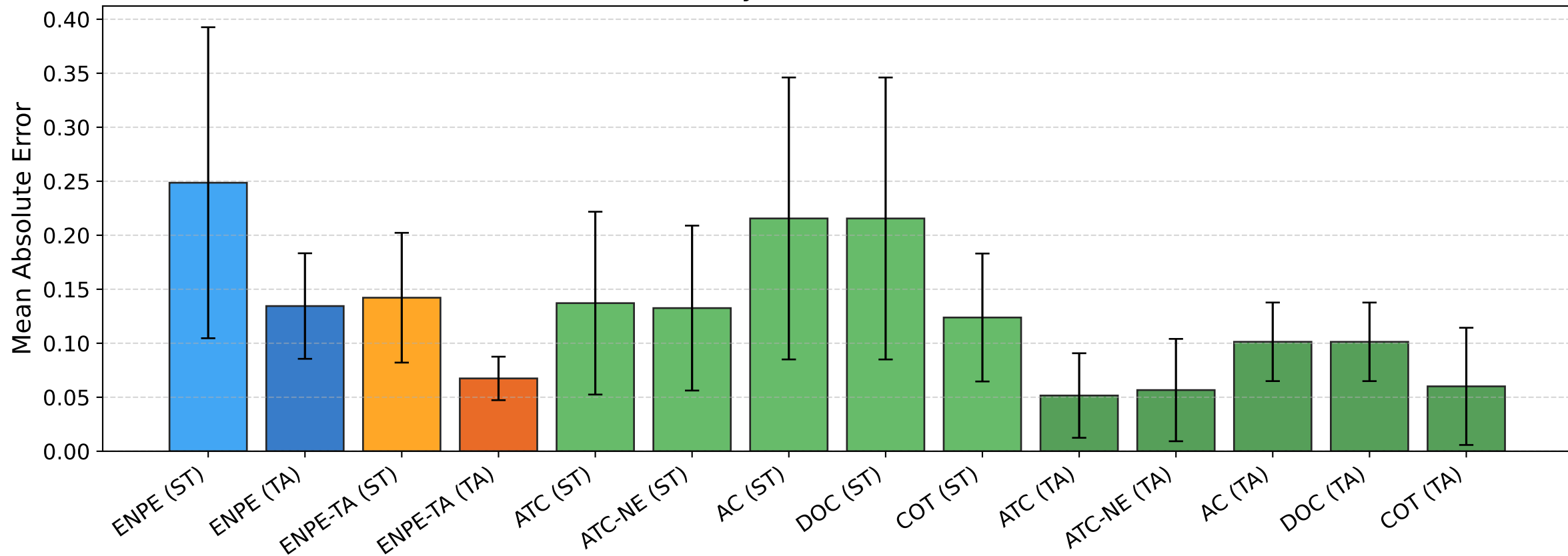
BREEDS entity30 — Mean Error [source]
