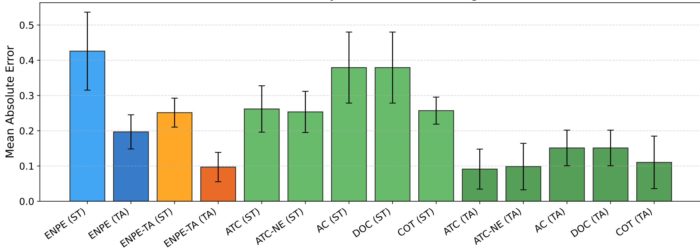
BREEDS entity30 — Mean Error [target]
