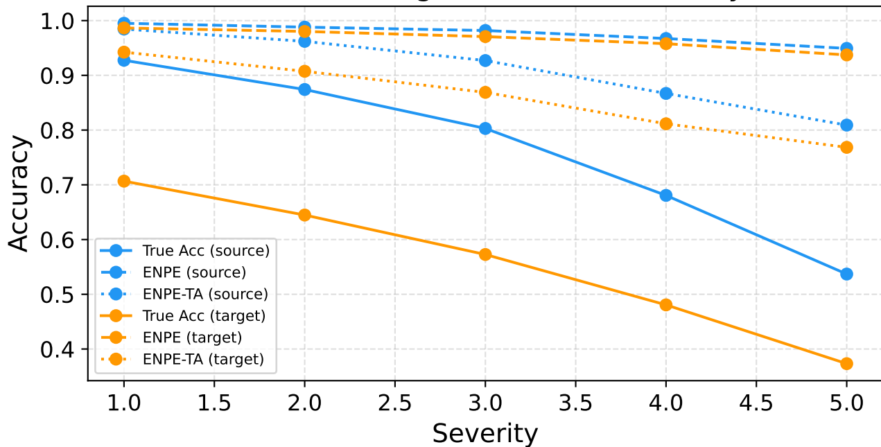
BREEDS living17 — Acc vs Severity
