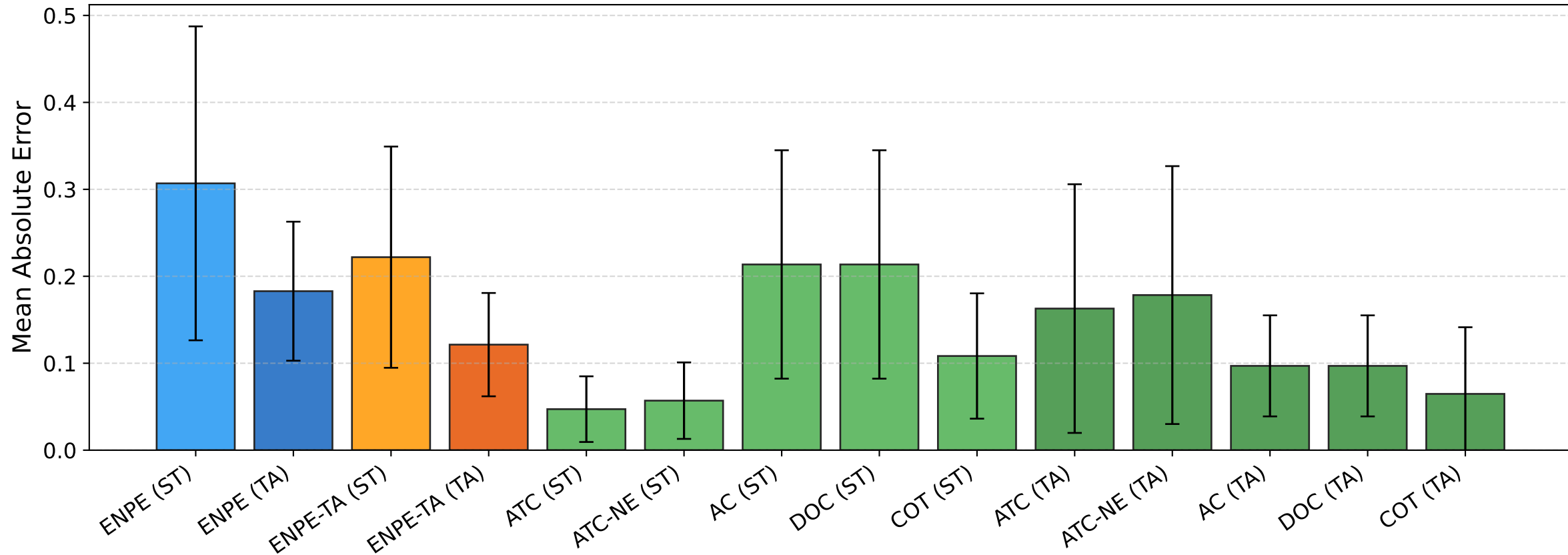
BREEDS living17 — Mean Error [all]
