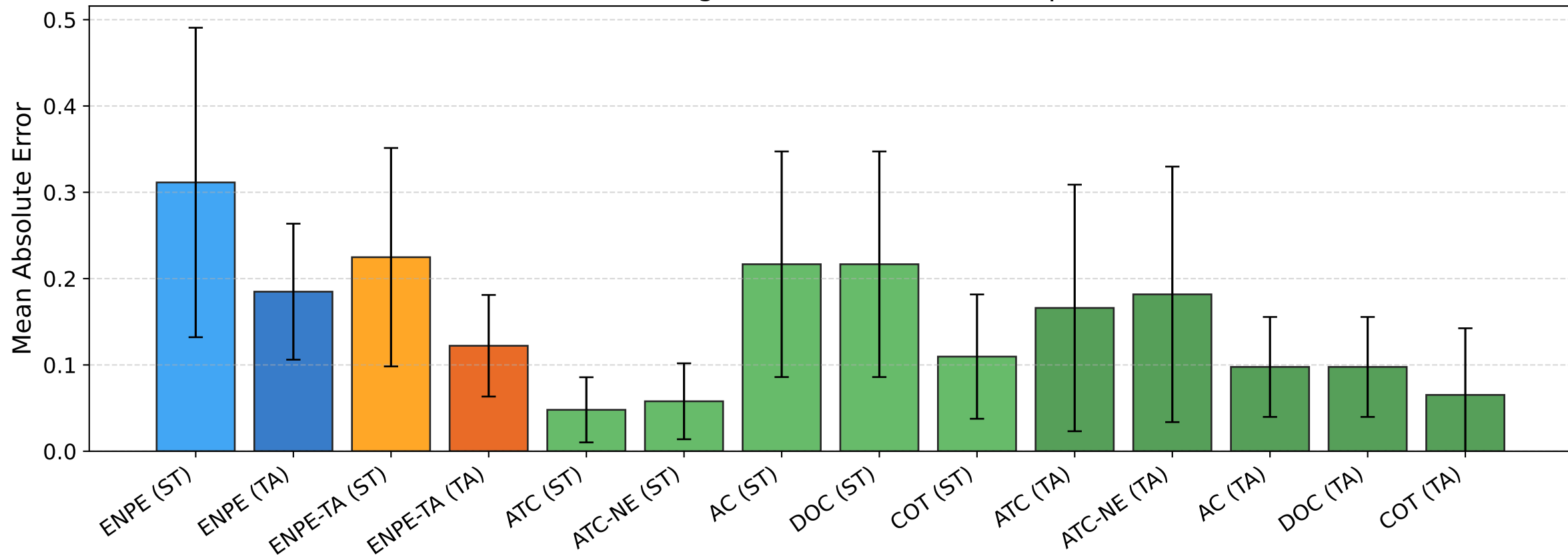
BREEDS living17 — Mean Error [corruptions]
