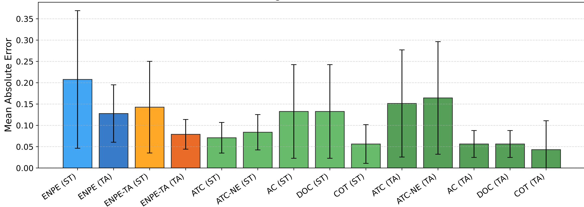
BREEDS living17 — Mean Error [source]
