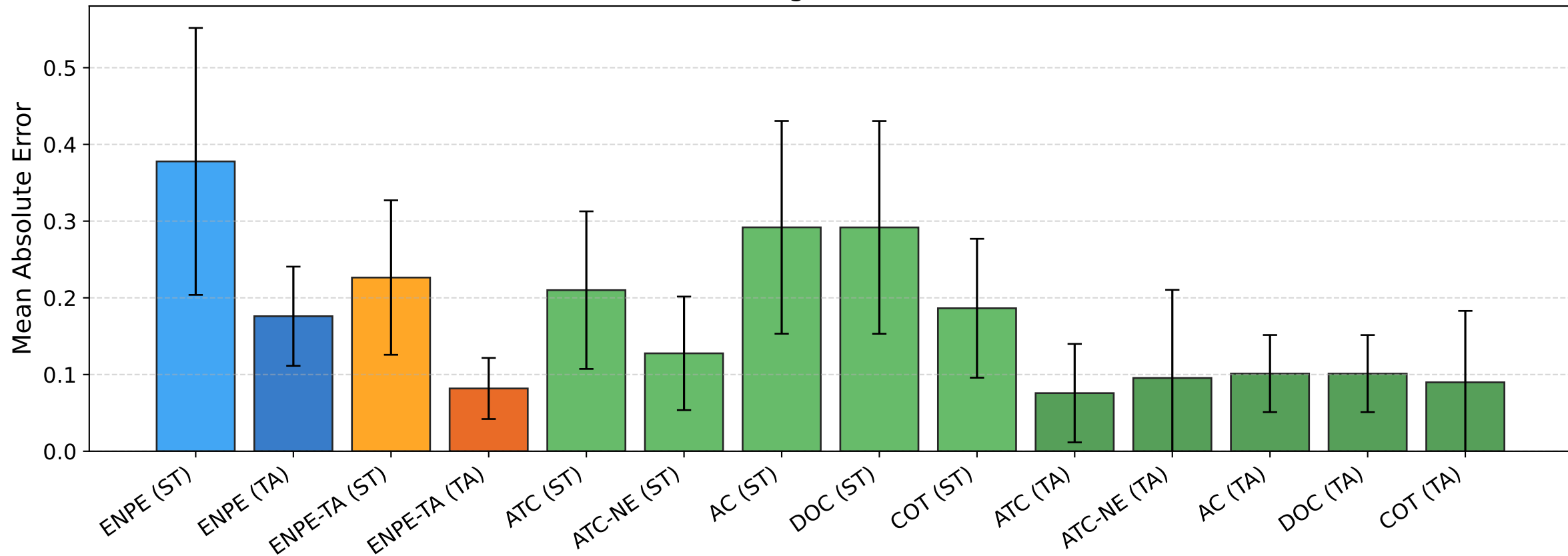
BREEDS nonliving26 — Mean Error [all]
