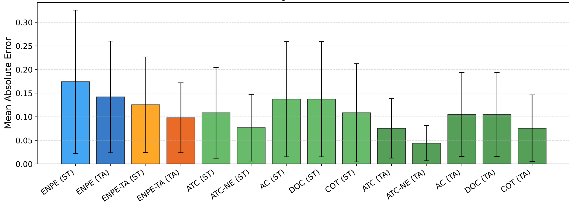
BREEDS nonliving26 — Mean Error [clean]
