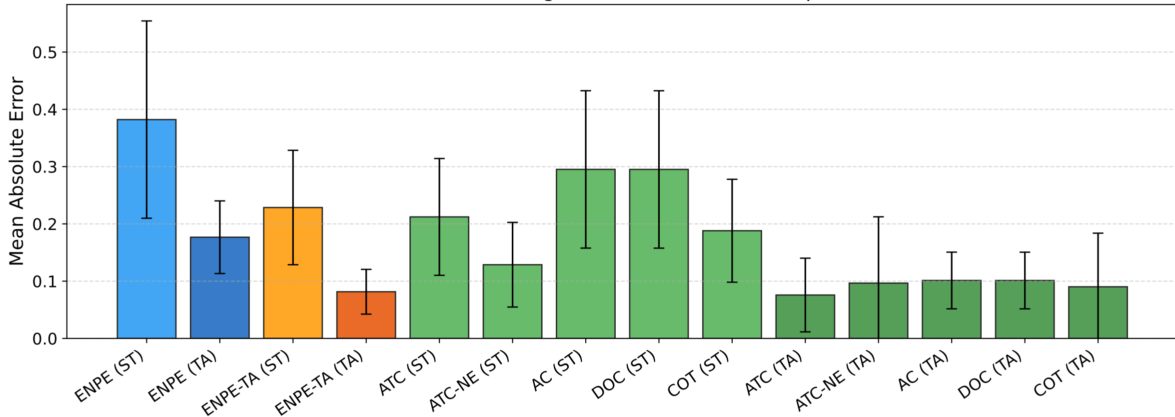
BREEDS nonliving26 — Mean Error [corruptions]
