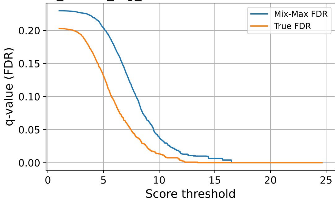
corr_source_fog_sev3 — FDR vs Score Threshold
