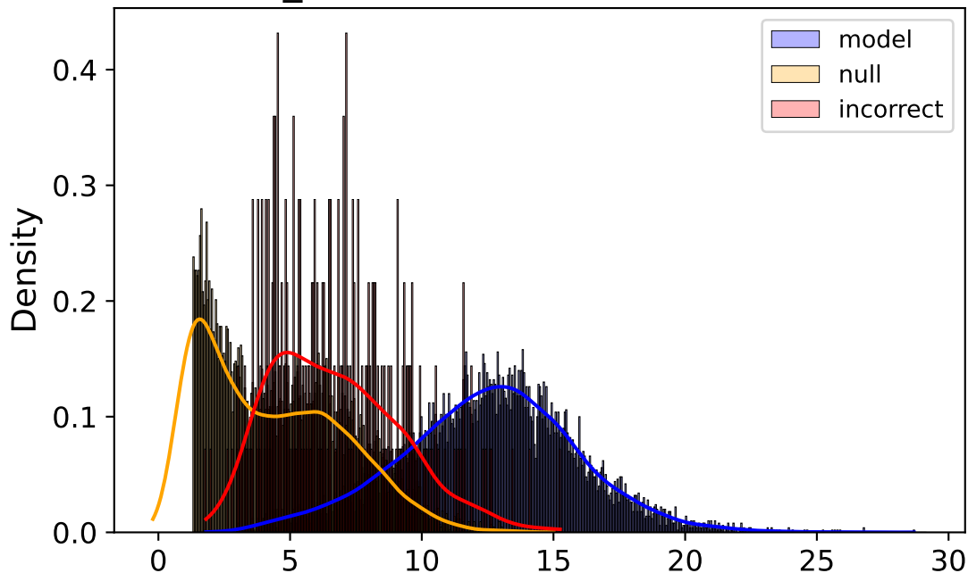
val_source — Score Distributions
