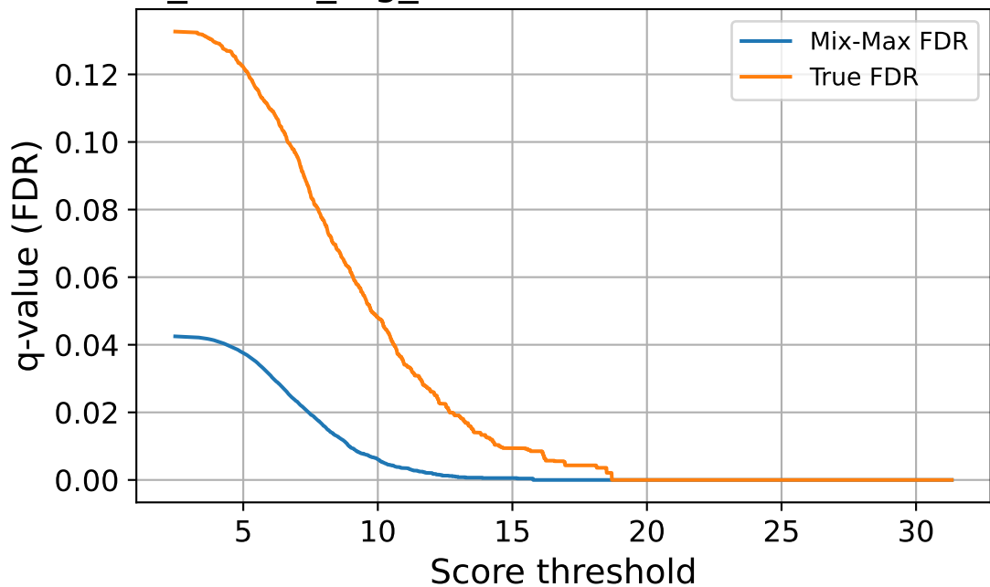
corr_source_fog_sev1 — FDR vs Score Threshold
