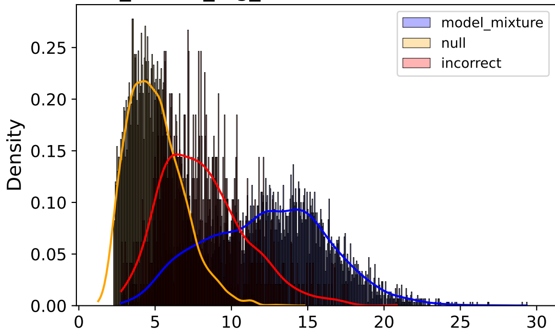
corr_source_fog_sev2 — Score Distributions
