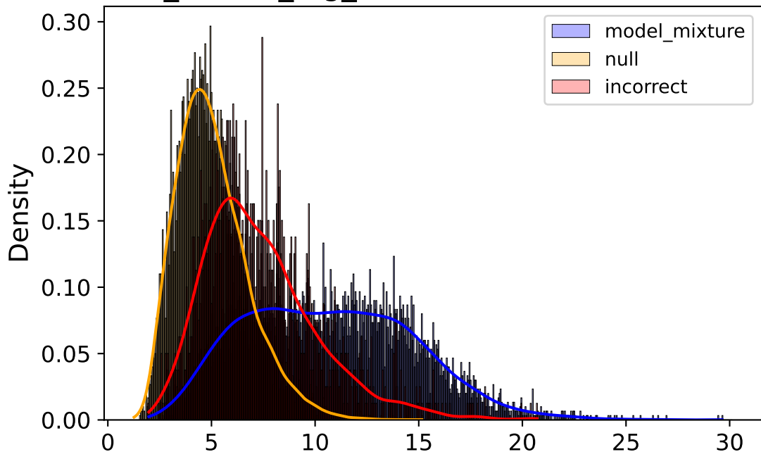
corr_source_fog_sev4 — Score Distributions
