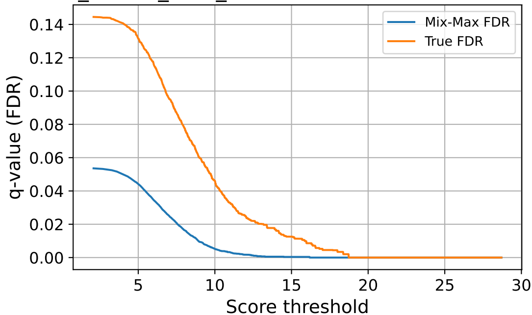
corr_source_frost_sev1 — FDR vs Score Threshold
