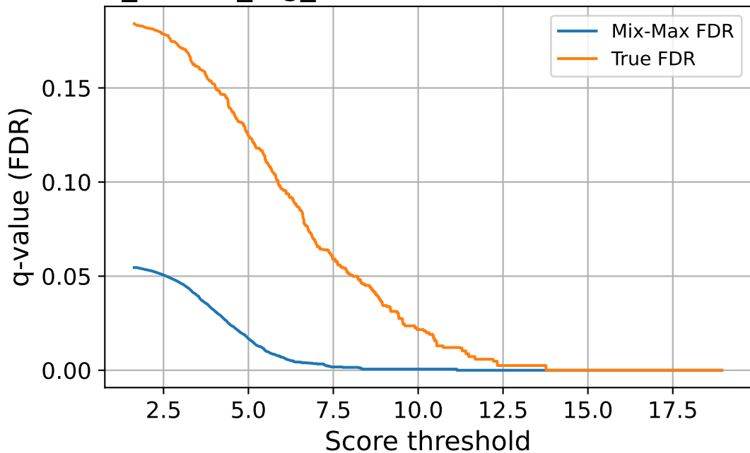
corr_source_fog_sev4 — FDR vs Score Threshold
