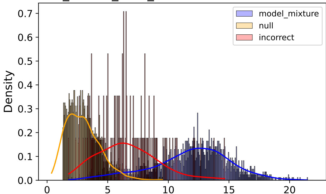
corr_source_frost_sev1 — Score Distributions
