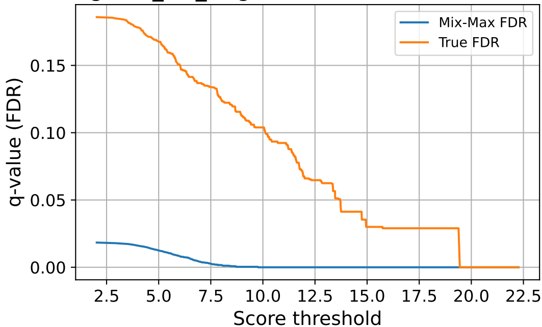
imagenet_val_target — FDR vs Score Threshold
