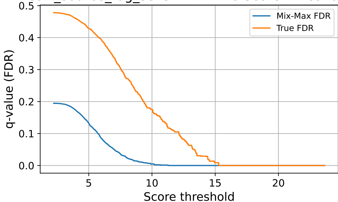
corr_source_fog_sev5 — FDR vs Score Threshold
