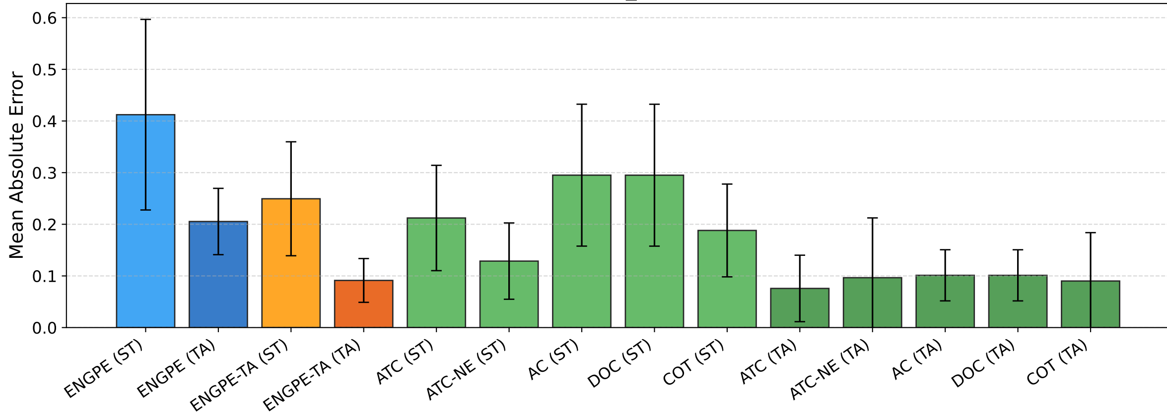
BREEDS nonliving26 [flows_24] — MAE [corruptions]
