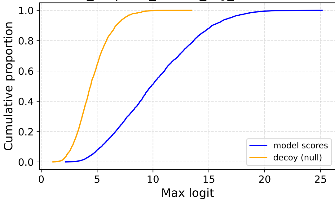
flows_24 | corr_source_fog_sev3 — ECDF
