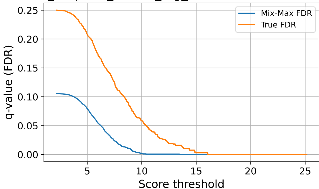
flows_24 | corr_source_fog_sev3 — FDR vs Threshold
