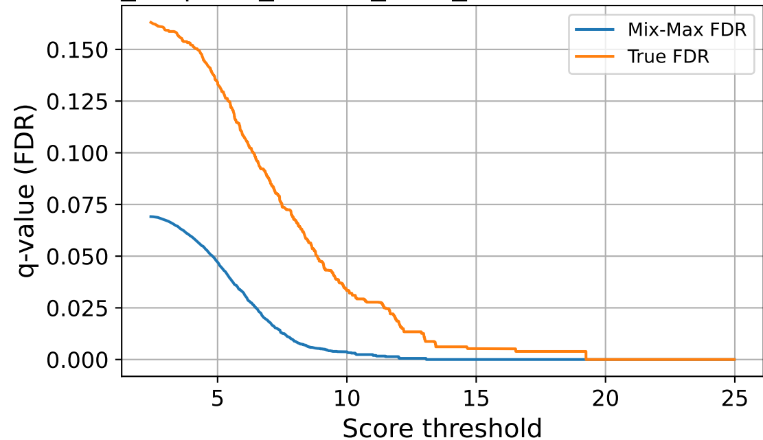
flows_24 | corr_source_frost_sev1 — FDR vs Thresh
