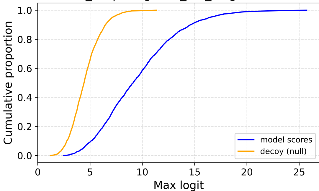
flows_24 | imagenet_val_target — ECDF
